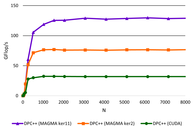
Fig. 7. Tuned SGEMM Performance on Intel UHD Graphics P630 [0x3e96]
