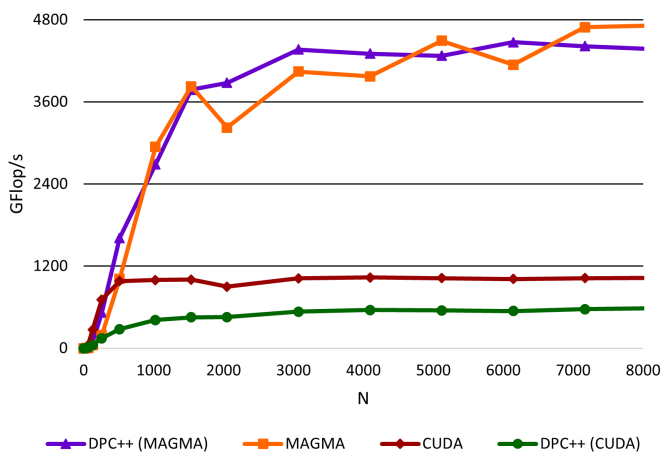
Fig. 5. SGEMM Performance on NVIDIA GeForce RTX 3060
