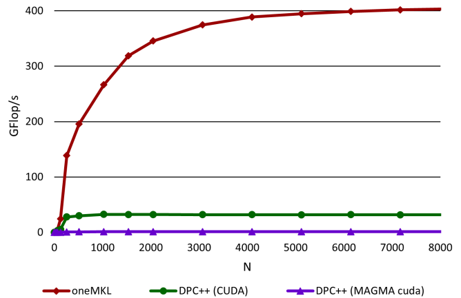
Fig. 6. Initial SGEMM Performance on Intel UHD Graphics P630 [0x3e96]
