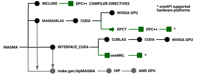
Fig. 1. Extended structure of MAGMA’s CUDA directories.
