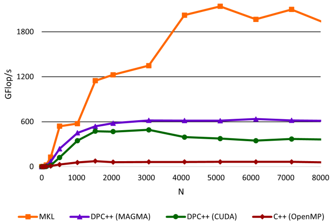
Fig. 4. SGEMM Performance on INTEL® XEON® CPU E5-2698 V4 20-Core Processor @ 2.20GHZ
