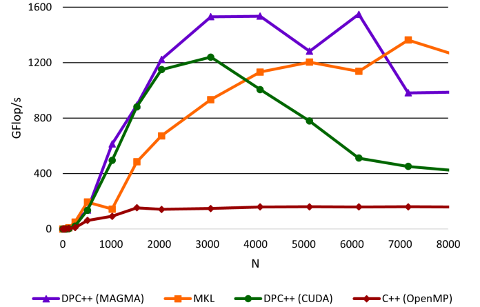
Fig. 3. SGEMM Performance on AMD EPYC 7742 64-Core Processor @ 2.25GHZ
